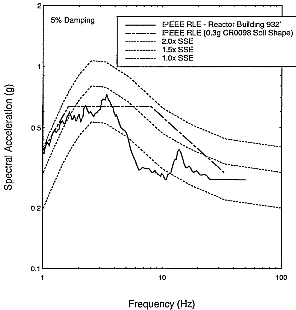
Figure 2. IPEEE RLE Floor Response Spectra for the Reactor Building
