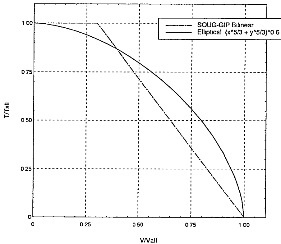
Figure 4. Comparison of Shear (V) / Tension (T) Interaction Curves
