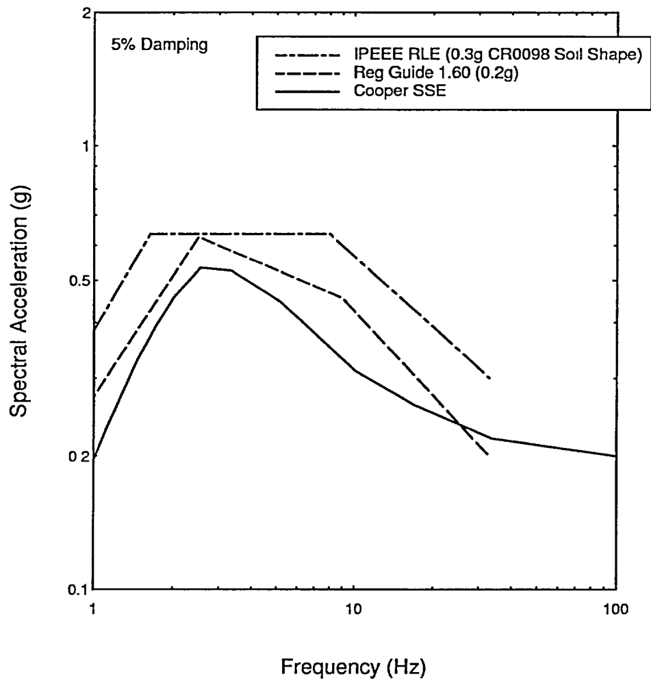
Figure 3. Comparison of Ground Response Spectra
